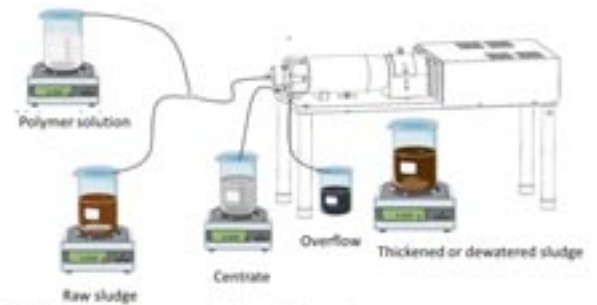
Fig. 1 - Lab screw centrifuge decanter
